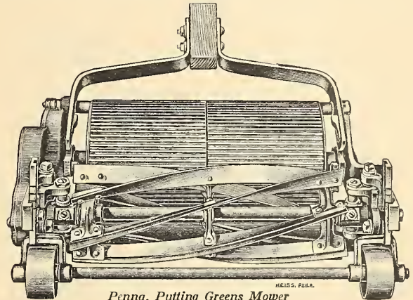
Penna. Putting Greens Mower
